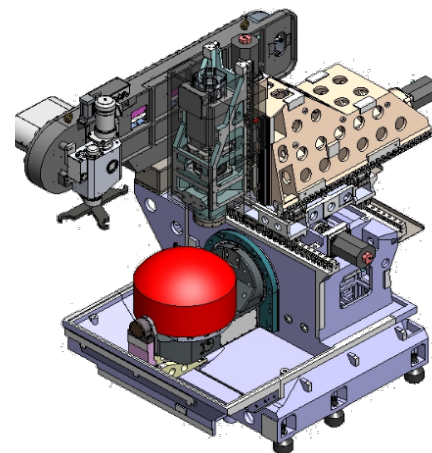
Machine Part with 3D print head retracting
